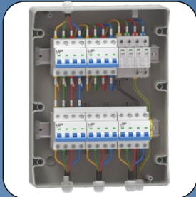
Surge Protection
